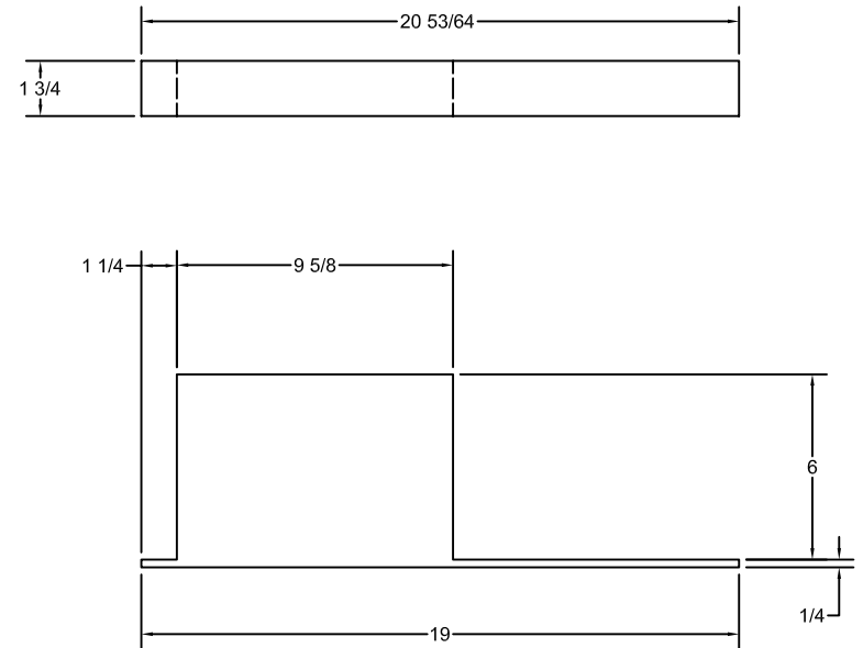
FOOT PRINT FOR RACK MOUNT DISPLAY ENCLOSURE
