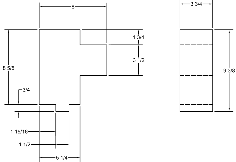
FOOT PRINT FOR SENSOR AND STANDARD DISPLAY ENCLOSURES
